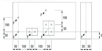
Picture 2: minimum spacing and edge distance
